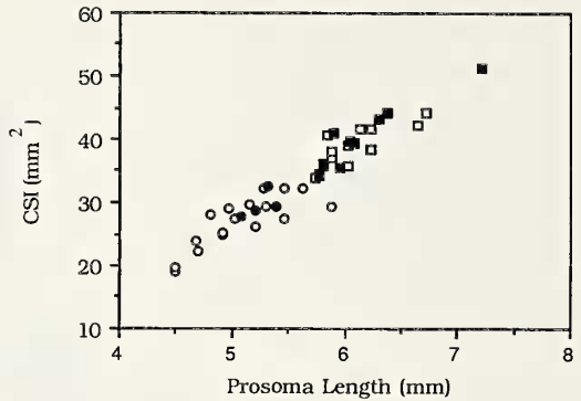
Figure 4.—Relationship between chela-size index (CSI = length of chela \times width) and prosoma length in adult females. Data have been separated into two putative instars (see text), sixth (circles) and seventh (squares). Females known to have given birth (filled symbols) occur in both instars.
